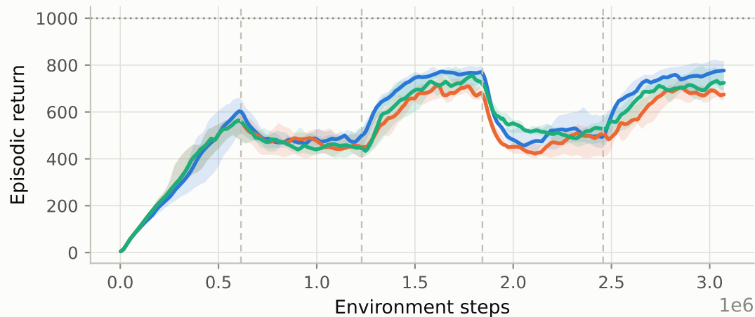
halfcheetah - 5 tasks of 614,400 steps (n=10)
