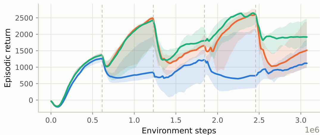
halfcheetah - 5 tasks of 614,400 steps (n=10)
