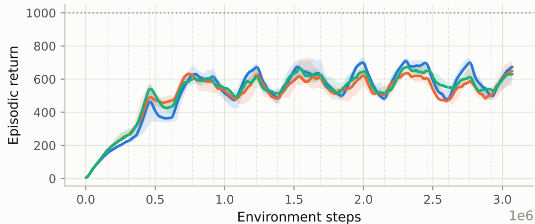
halfcheetah - 20 tasks of 153,600 steps (n=10)
