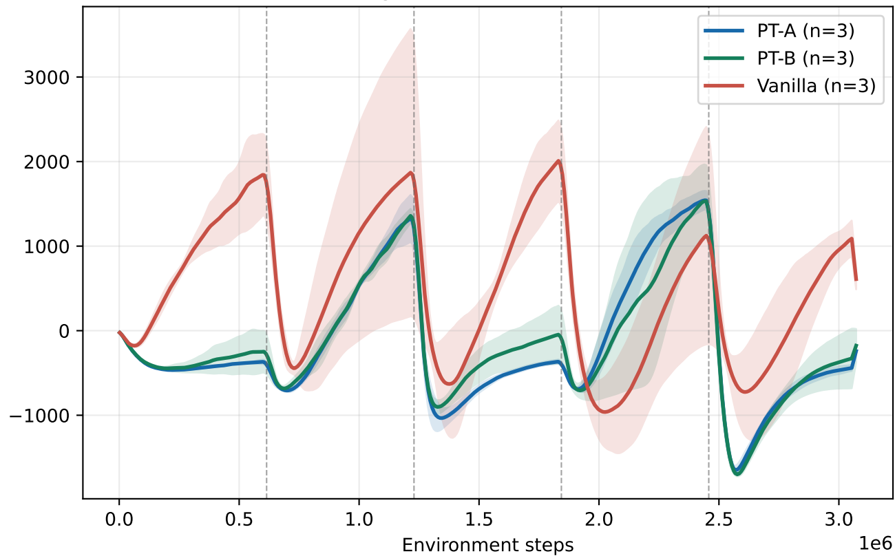
Mean boundary drop
