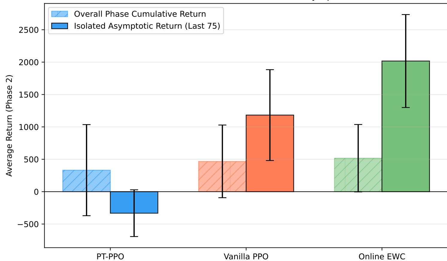
Phase 2: Overall Cumulative vs. Isolated Asymptotic Return
