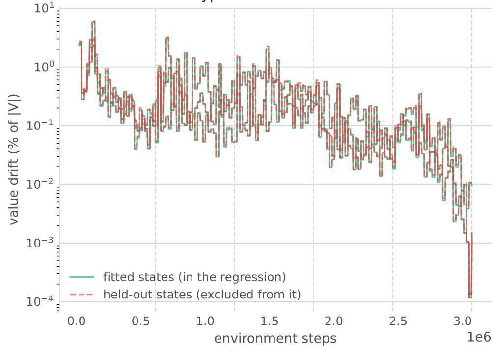
(b) Round 6 — held-out tracks fitted the memorisation hypothesis is falsified
