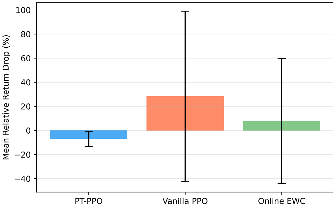
Relative Task-Switch Return Drop
