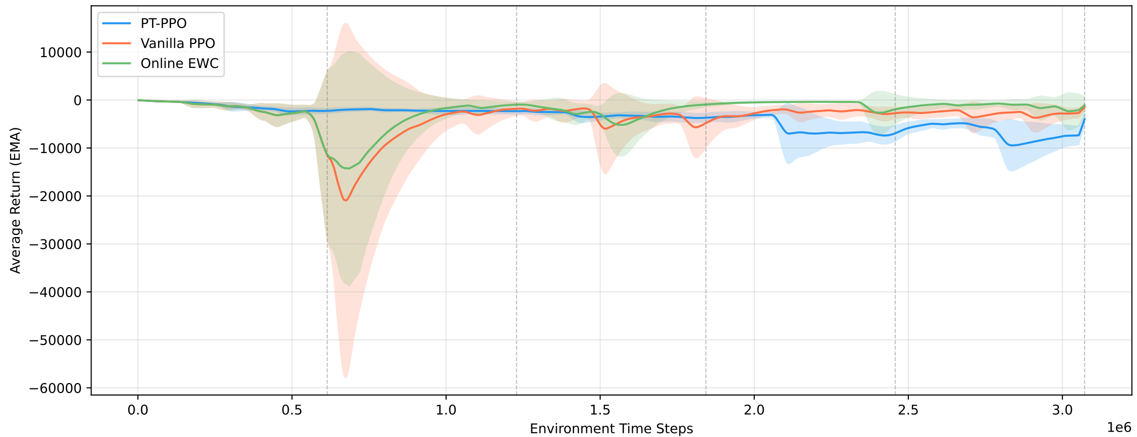
Continual HalfCheetah: PT-PPO vs Vanilla PPO vs Online EWC
