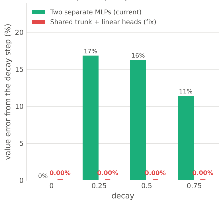
(c) Parameter scaling is not output scaling exact for any decay only with linear heads
