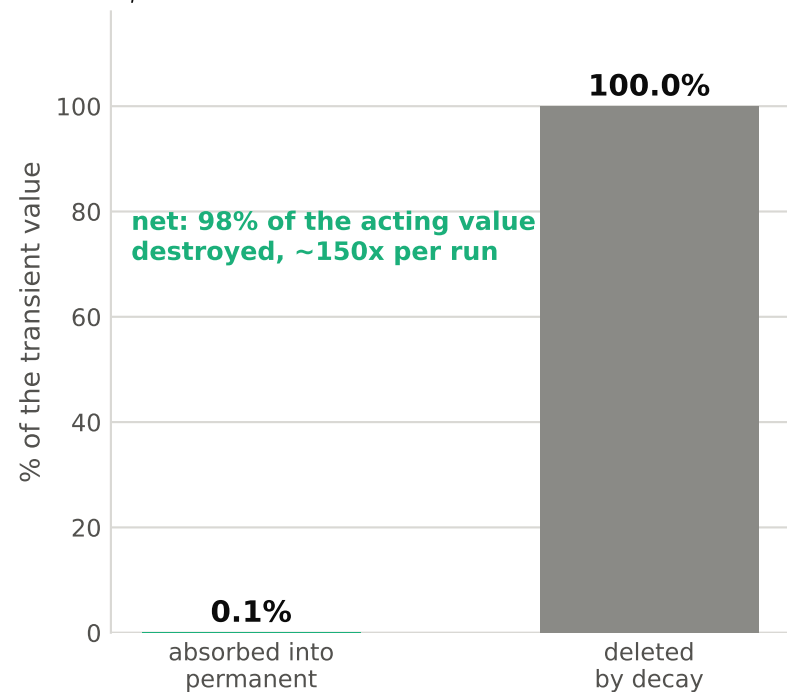
(a) One consolidation, production settings lr_{perm}=1e-5 , SGD, 1 epoch (320 steps)
