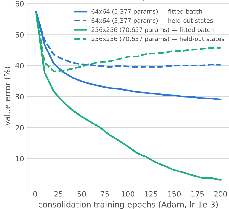
(b) The target IS fittable — but only on the batch held-out error does not improve
