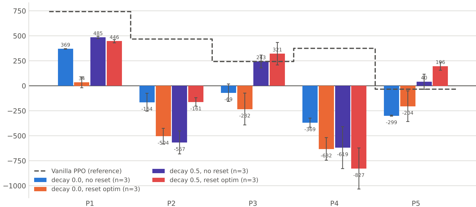
Round 7: transient decay \times resetting the transient's optimiser state the reset helps at decay 0.5 and hurts at decay 0.0 — the reverse of the stale-momentum prediction
