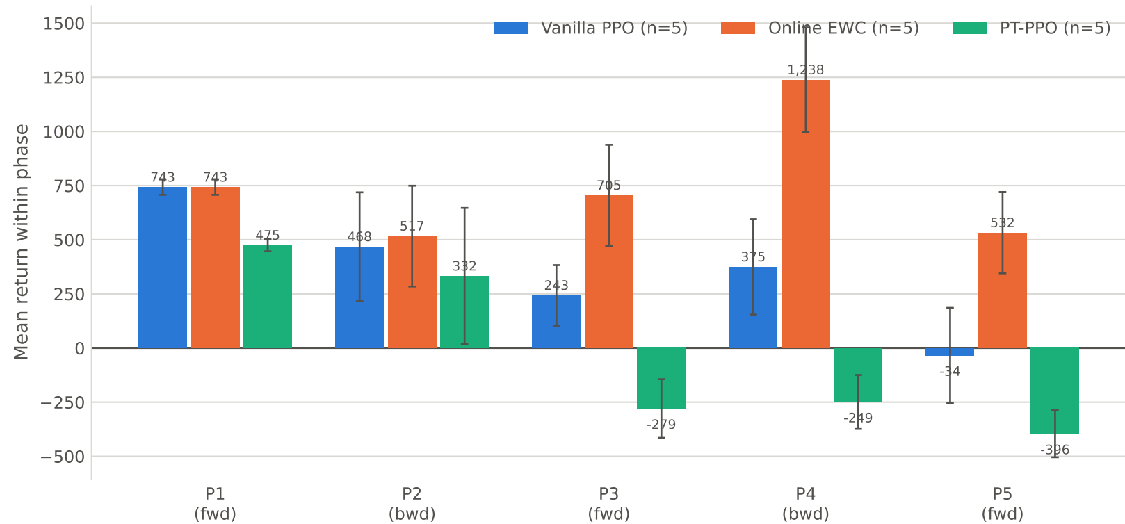
Continual HalfCheetah: per-phase mean return (error bars = SEM over seeds)
