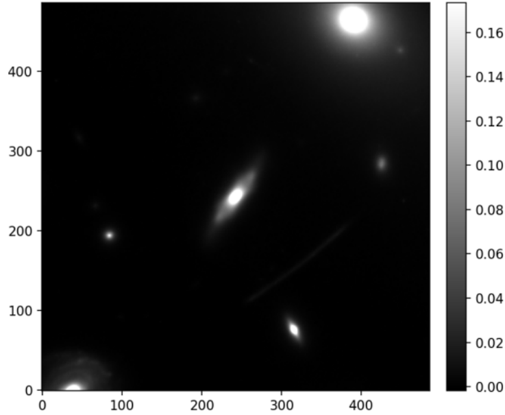
Residual: observed - model (RMS=2.364e-02)
