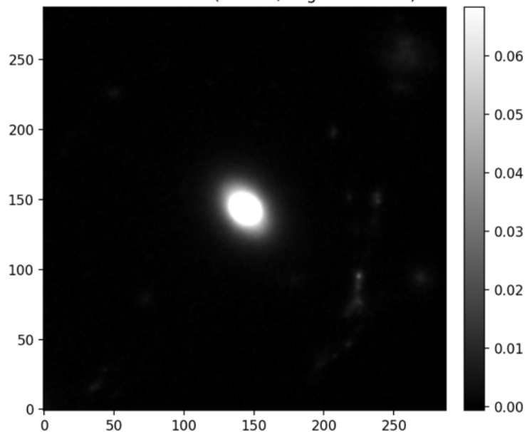
Residual: observed - model (RMS=6.153e-03)
