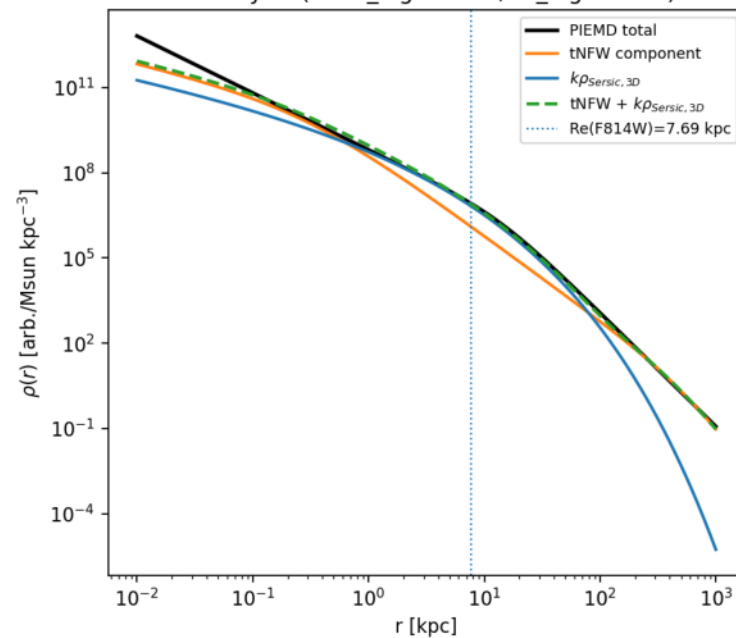
Density fit (rmse_log=0.220, r2_log=0.999)
