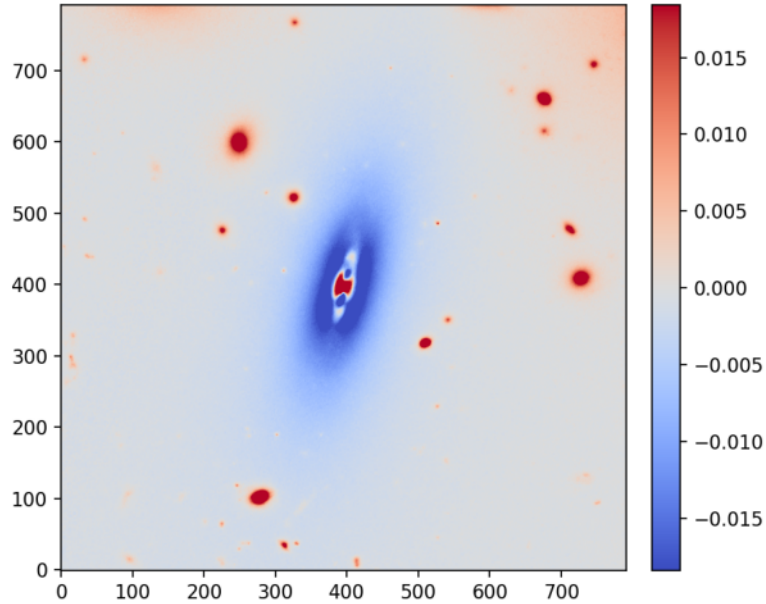
Residual: observed - model (RMS=5.458e-03)
