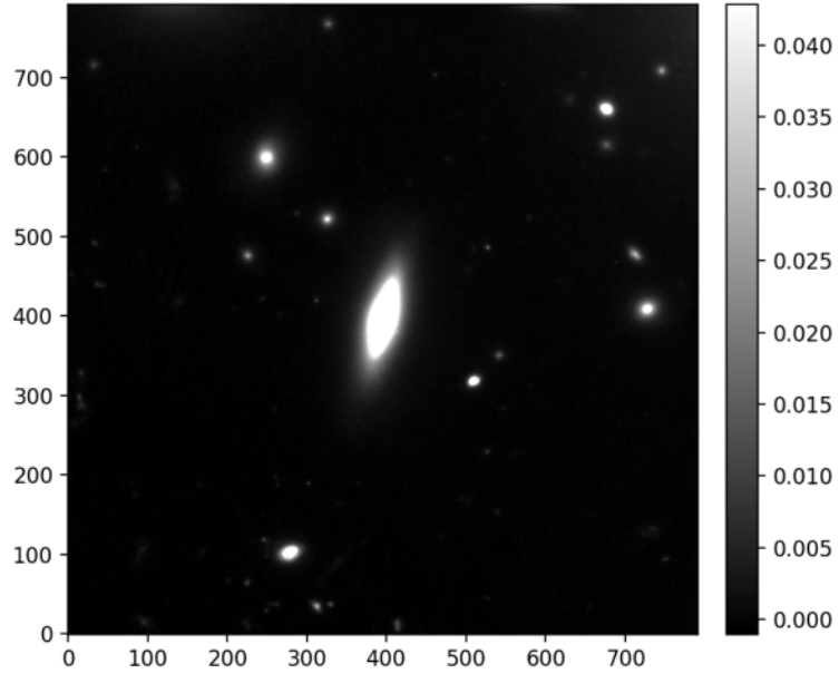
Residual: observed - model (RMS=5.458e-03)
