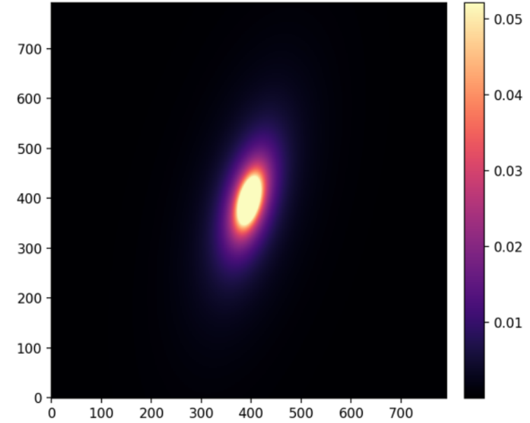
Density fit (rmse_log=0.771, r2_log=0.989)
