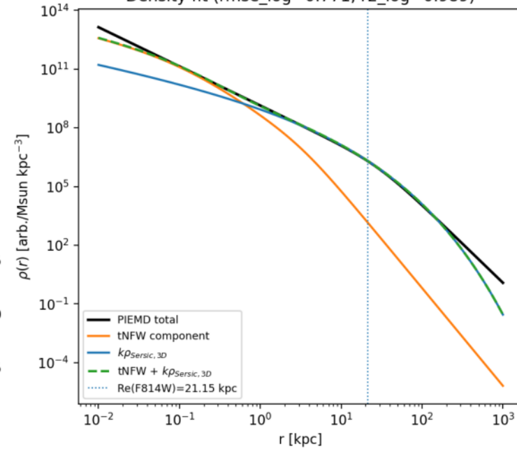
Density fit (rmse_log=0.771, r2_log=0.989)
