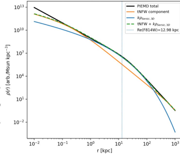
Density fit (rmse_log=0.163, r2_log=1.000)
