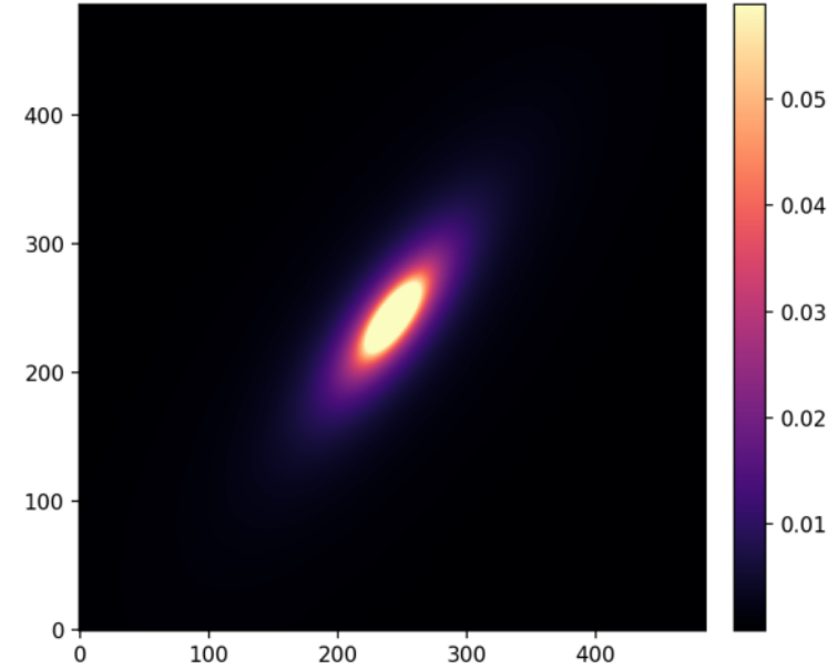
Density fit (rmse_log=0.163, r2_log=1.000)
