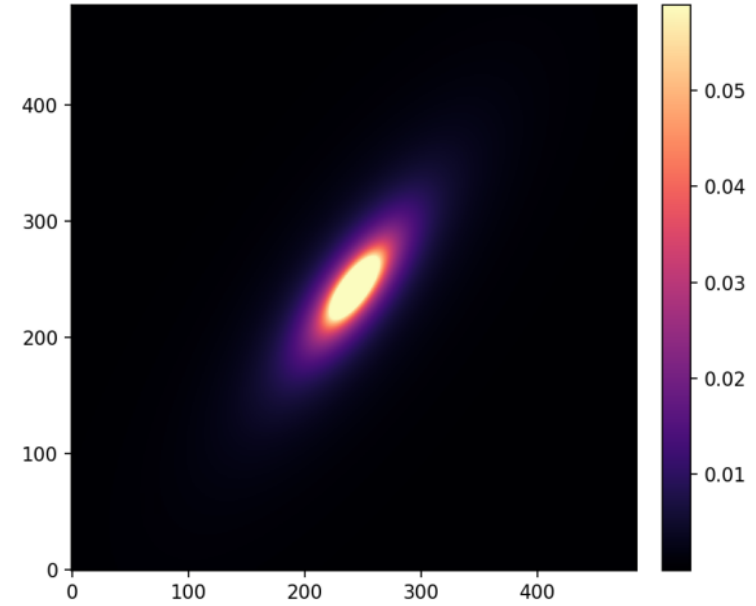
Surface-density fit (rmse_log=0.420, r2_log=0.987)
