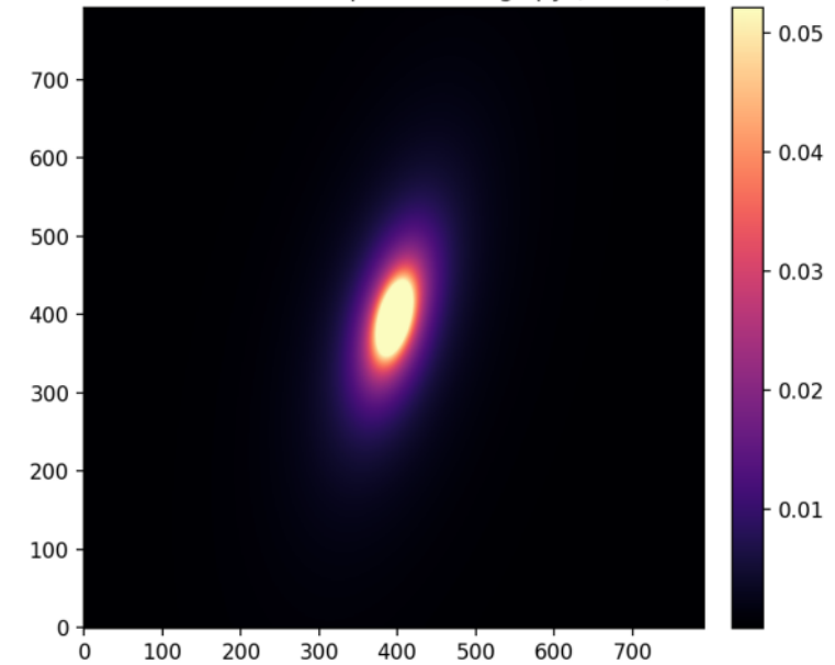
Surface-density fit (rmse_log=0.193, r2_log=0.997)
