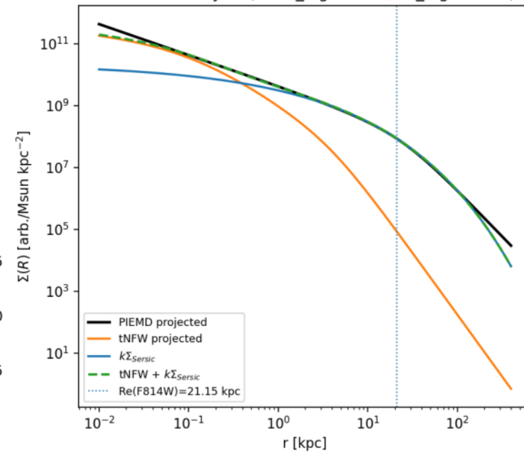
Surface-density fit (rmse_log=0.193, r2_log=0.997)
