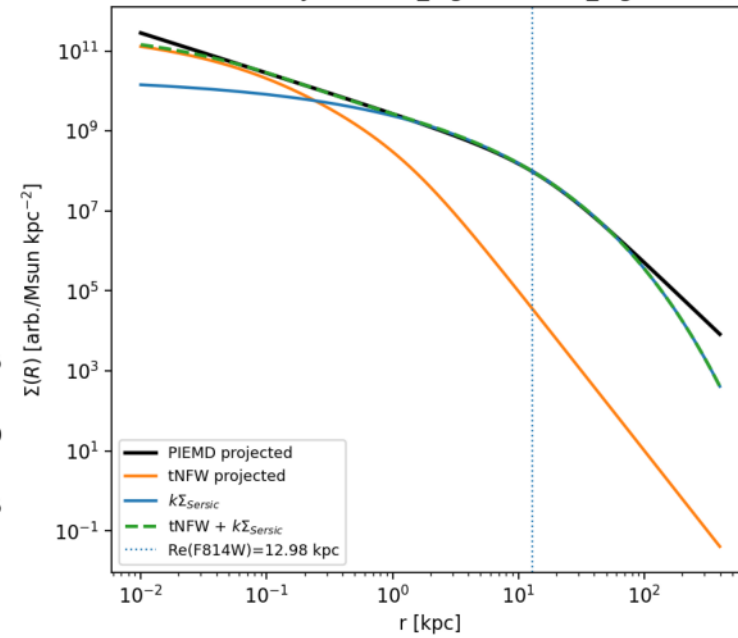
Surface-density fit (rmse_log=0.420, r2_log=0.987)
