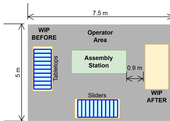
FIGURE 38: ASSEMBLY WORKSTATION
