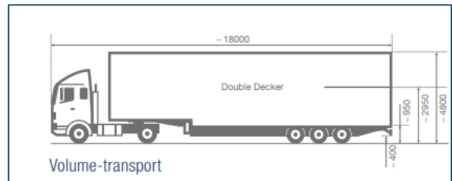
FIGURE 3: TRUCK DIMENSIONS
