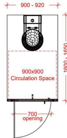
FIGURE 6: STANDARD BATHROOM STALL LAYOUT
