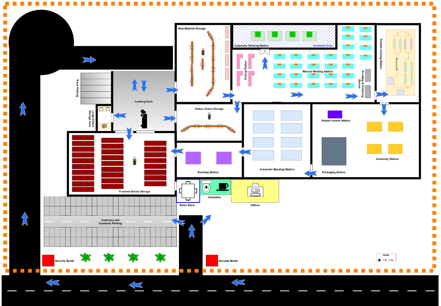
FIGURE 66: MFP MATERIAL AND PEOPLE FLOW
