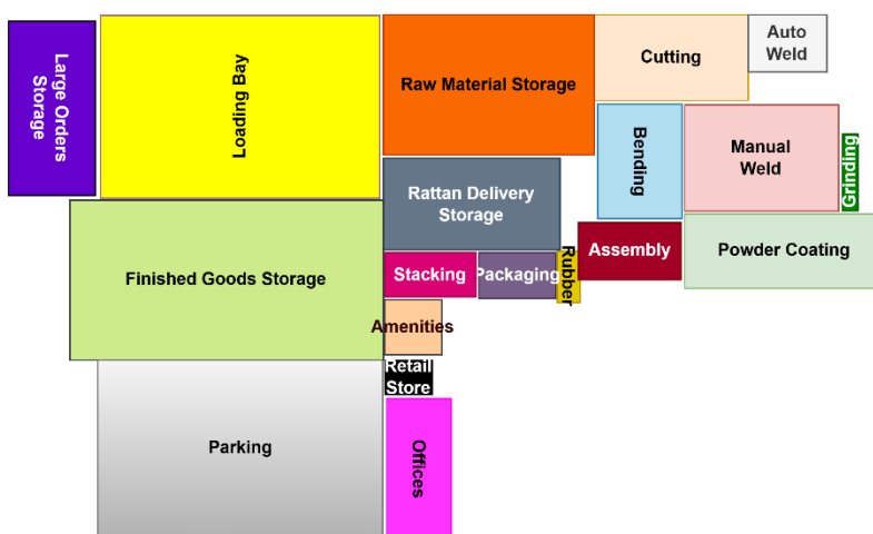
FIGURE 64: ALTERNATIVE LAYOUT
