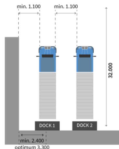
FIGURE 1: LOADING BAY STANDARD DIMENSIONS (IN MM)
