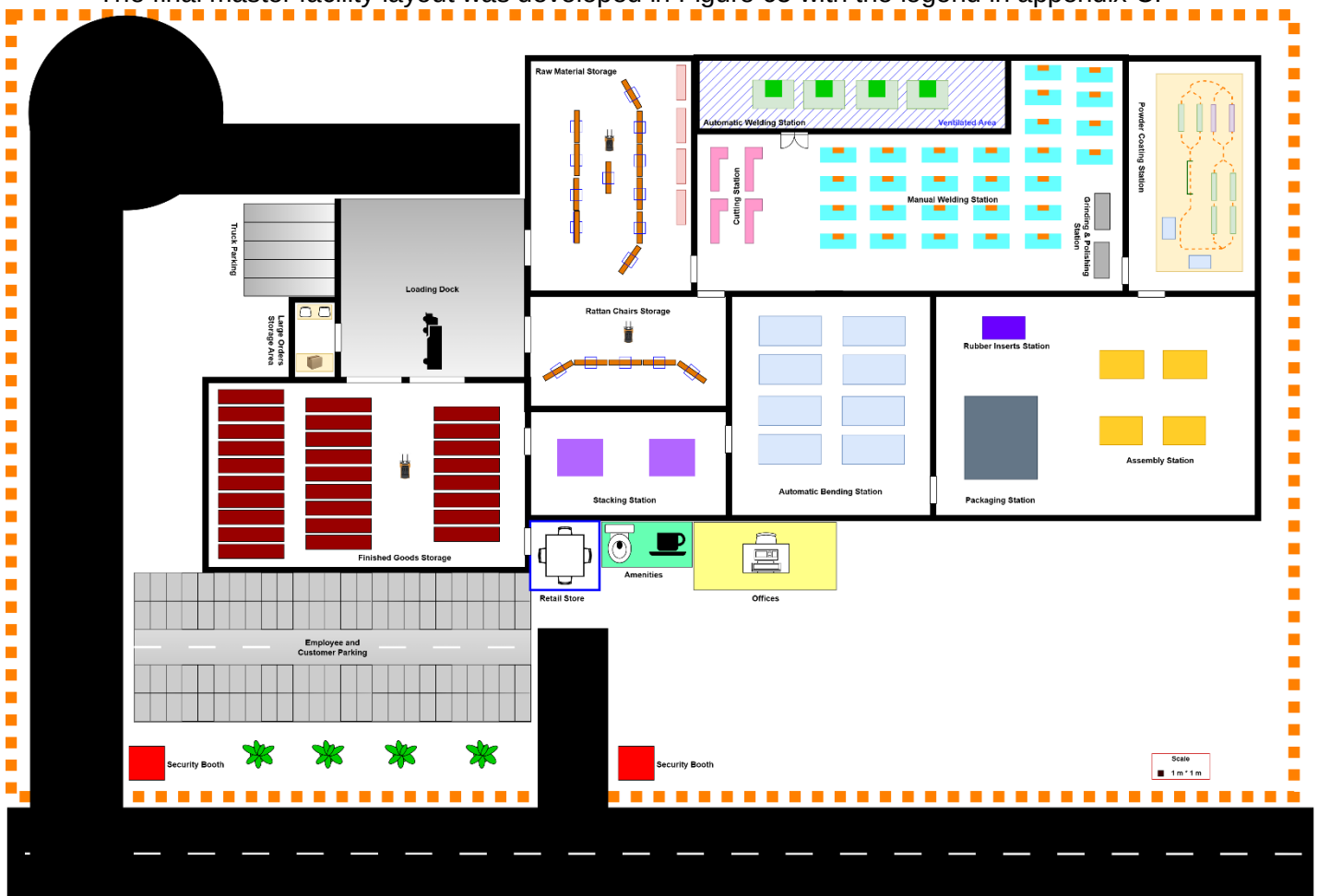
FIGURE 65: THE FINAL MFP LAYOUT
