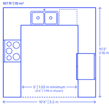
FIGURE 5: STANDARD KITCHEN LAYOUT
