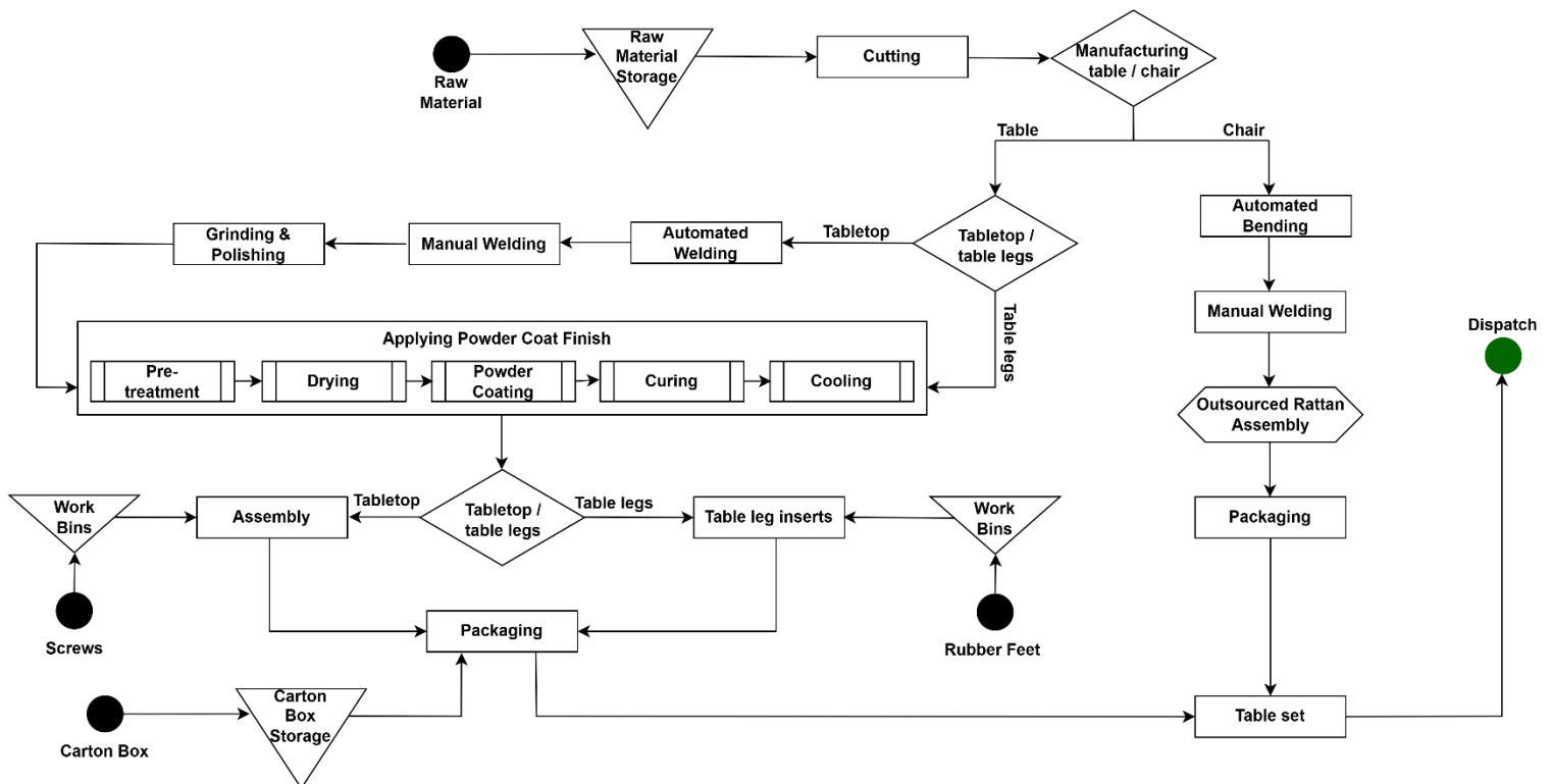
FIGURE 7: PROCESS FLOW DIAGRAM
