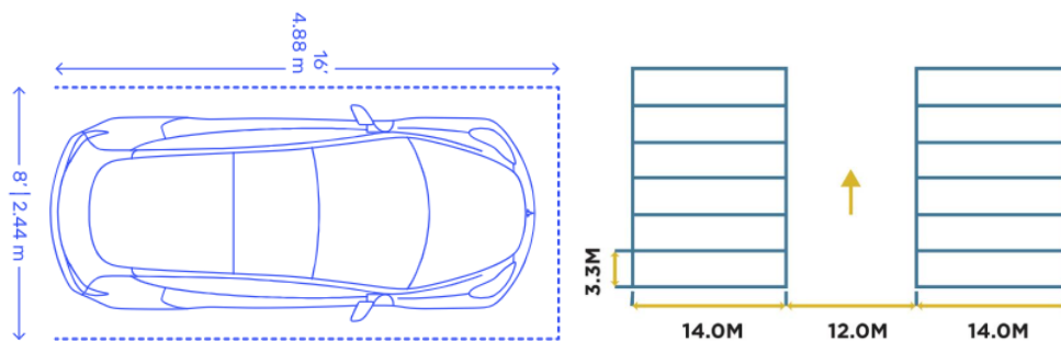
FIGURE 4: STANDARD VEHICLE AND TRUCK PARKING
