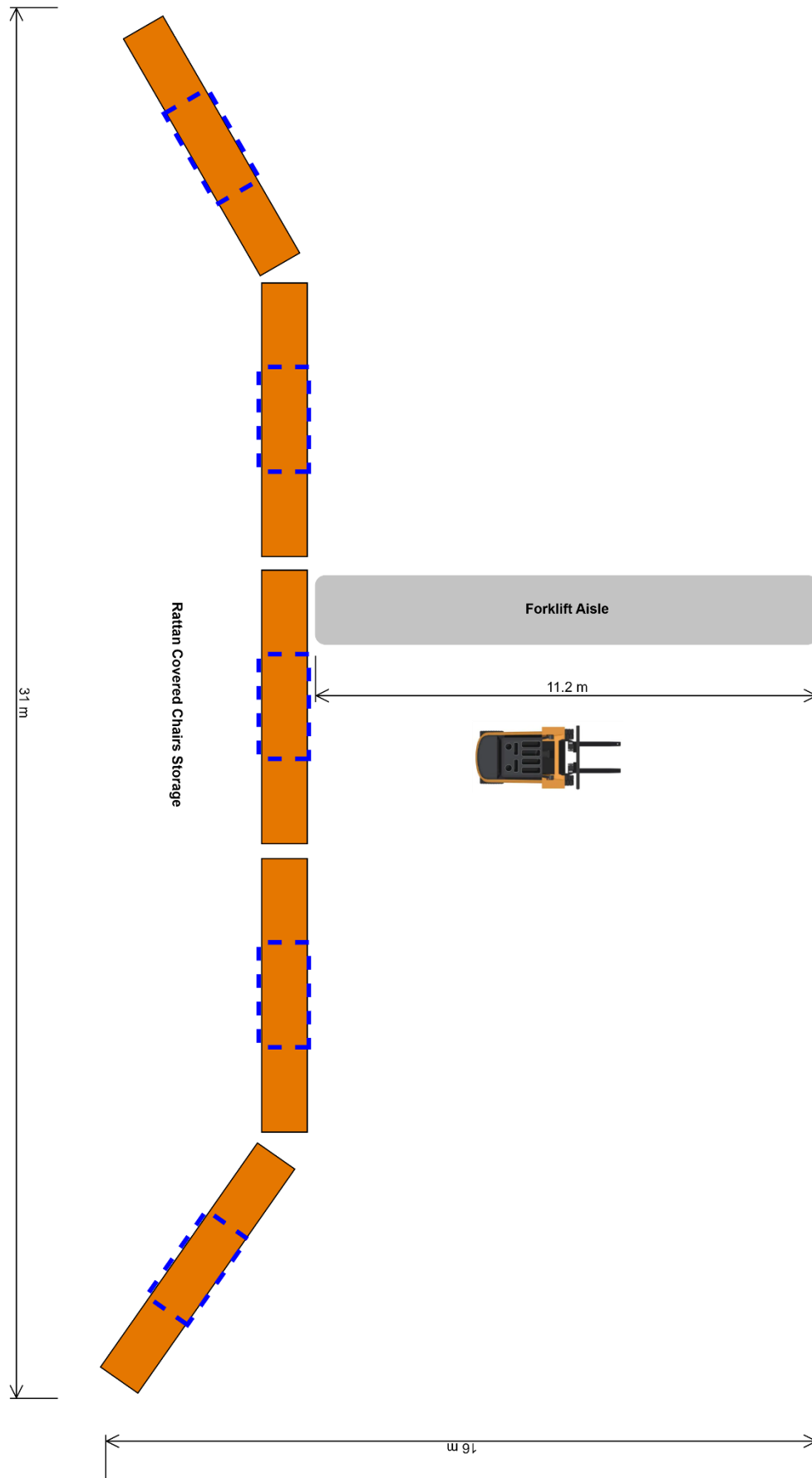
FIGURE 68: ENLARGED RATTAN PRODUCTS LAYOUT
