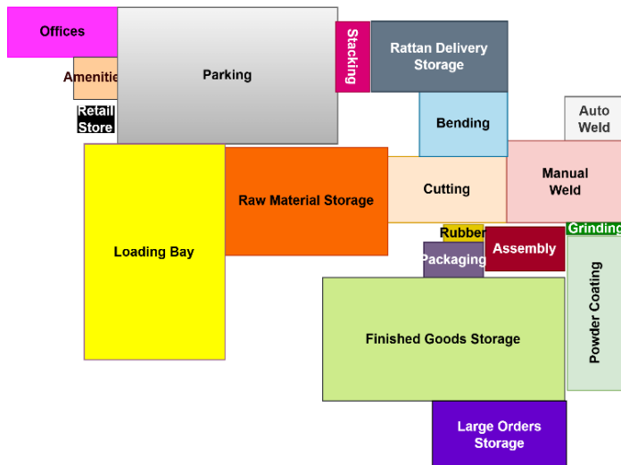
FIGURE 62: ALTERNATIVE LAYOUT 1
