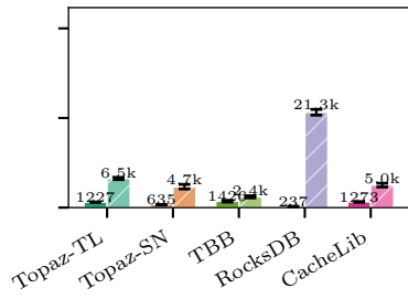
YCSB-C (64B)
