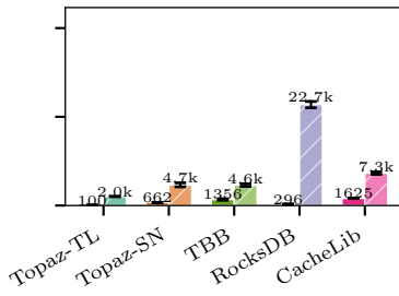
YCSB-B (64B)
