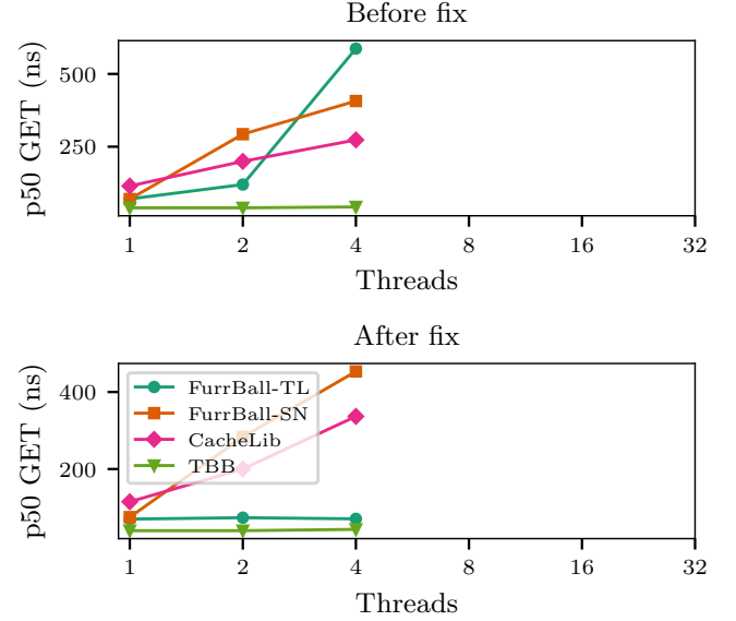
Figure 4. Thread scaling on c6a (4 NUMA nodes) before and after per-node stat fix. Top: before. Bottom: after. Before: FurrBallTL degrades 6.6\times at 4T. After: flat at 71 ns.
