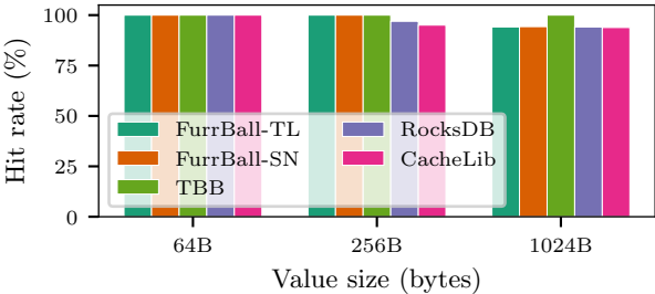
YCSB-B, 2T, 32MB cache
