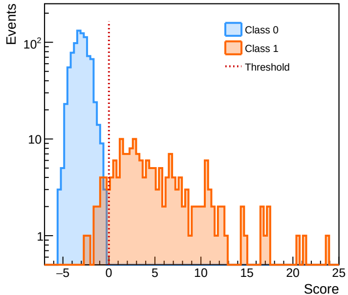
Keras Score Distribution
