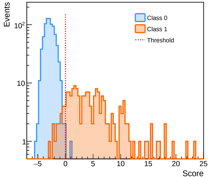
RTL Score Distribution
