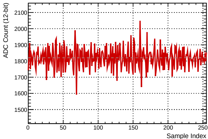
Ch 3 | Event #50 | Label: SIGNAL | CNN Score: 5139
