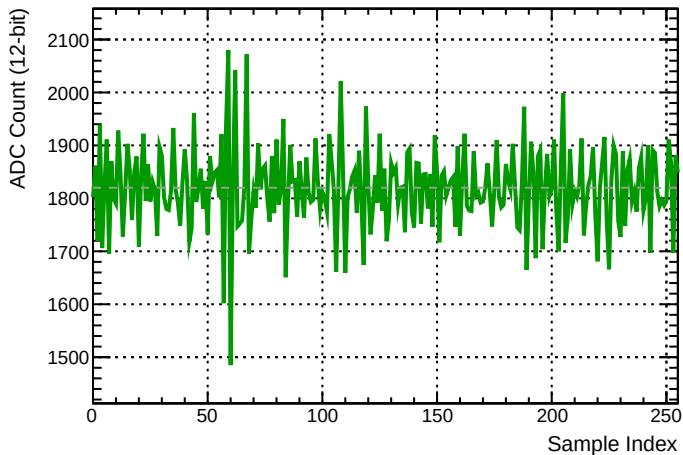
Ch 2 | Event #50 | Label: SIGNAL | CNN Score: 5139
