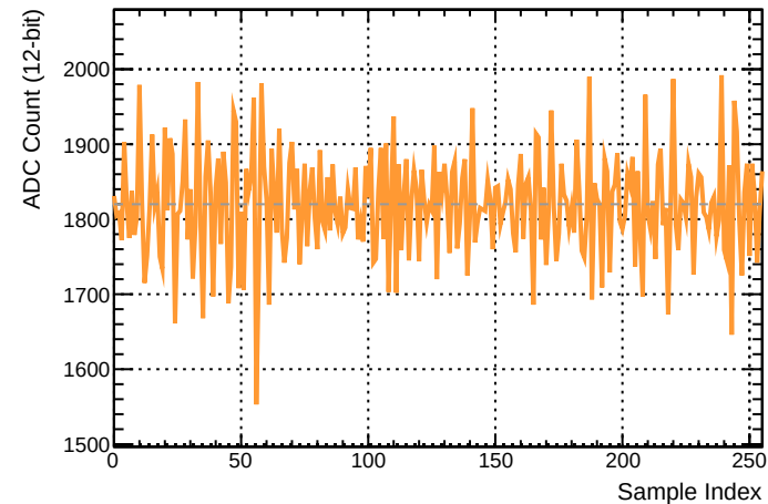
Ch 3 | Event #905 | Label: Background | CNN Score: 5515
