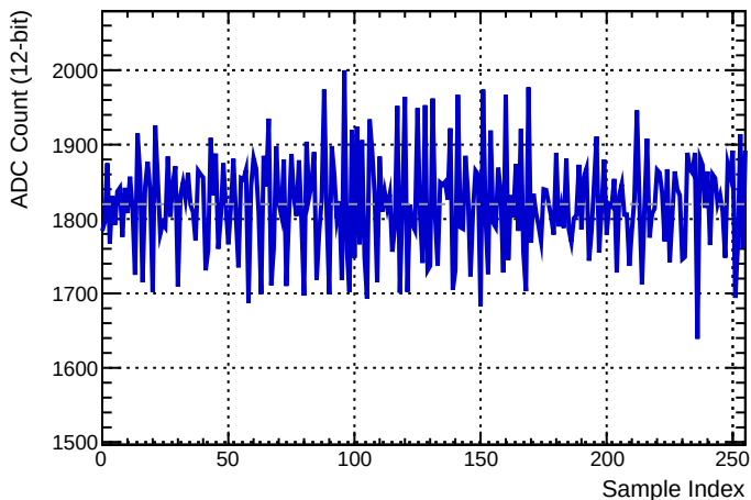
Ch 2 | Event #905 | Label: Background | CNN Score: 5515
