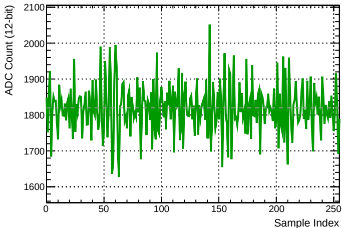
Ch 2 | Event #39 | Label: SIGNAL | CNN Score: 5227
