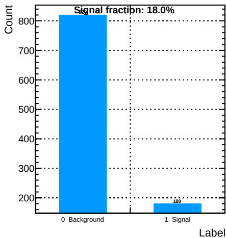
Label Distribution
