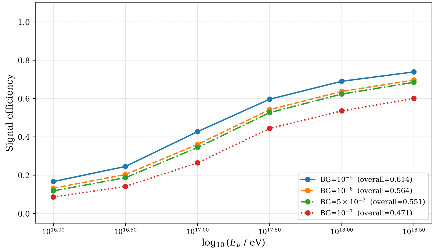
Efficiency vs. Energy — HGQPhase2ModelMini (mini_es0)
