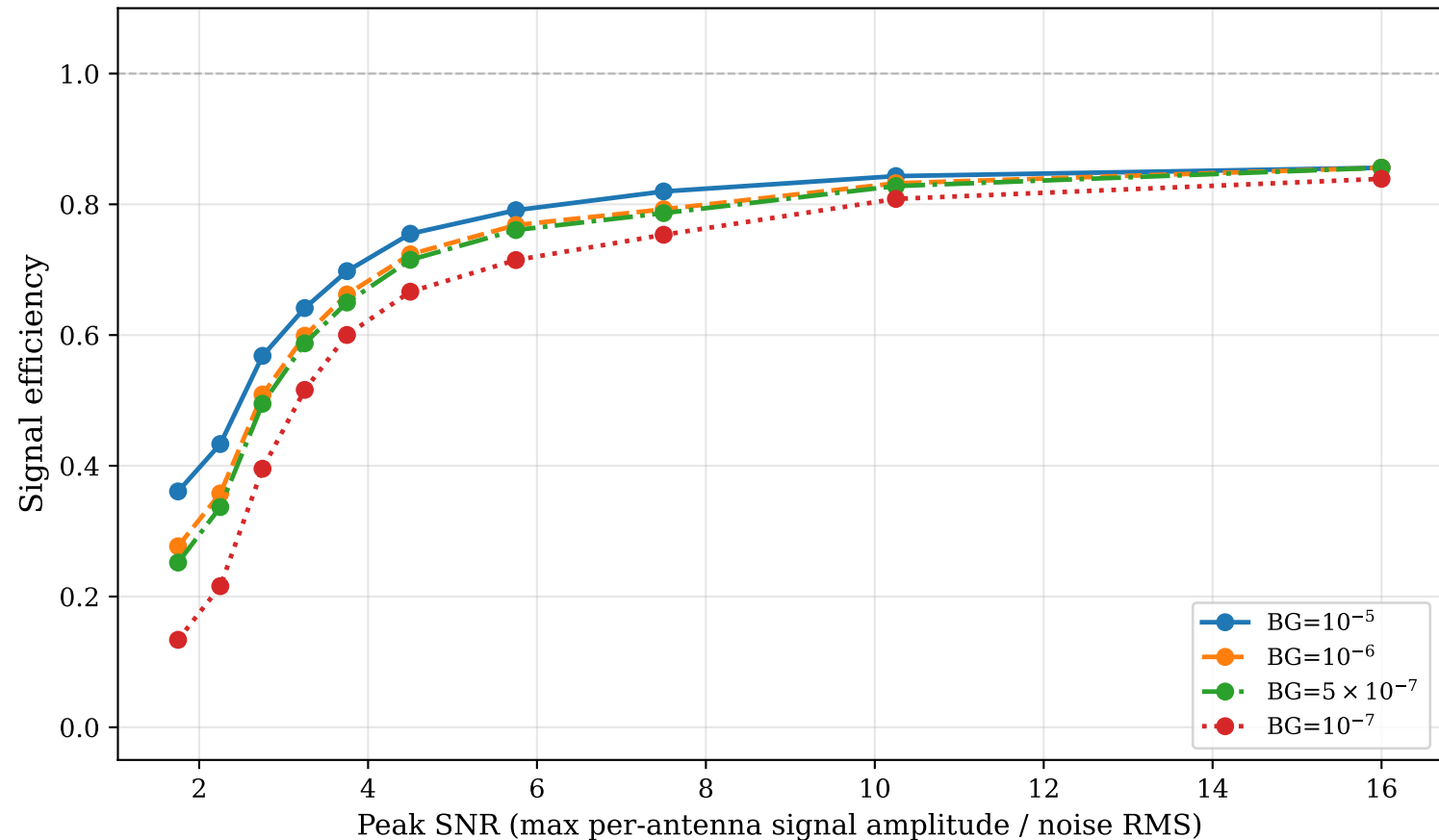
Efficiency vs. SNR — HGQPhase2ModelMini (mini_es0)
