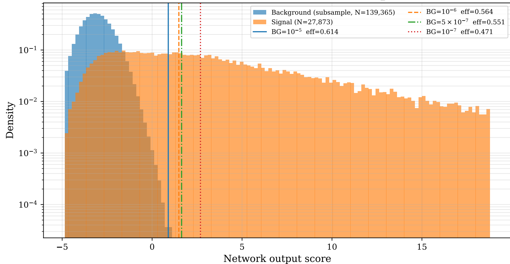
Score distributions — HGQPhase2ModelMini (mini_es0)
