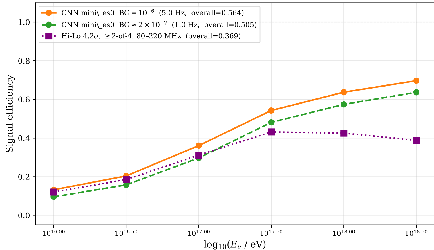
Efficiency vs. Energy — mini\_es0 CNN vs. Hi-Lo 4.2 \sigma reference
