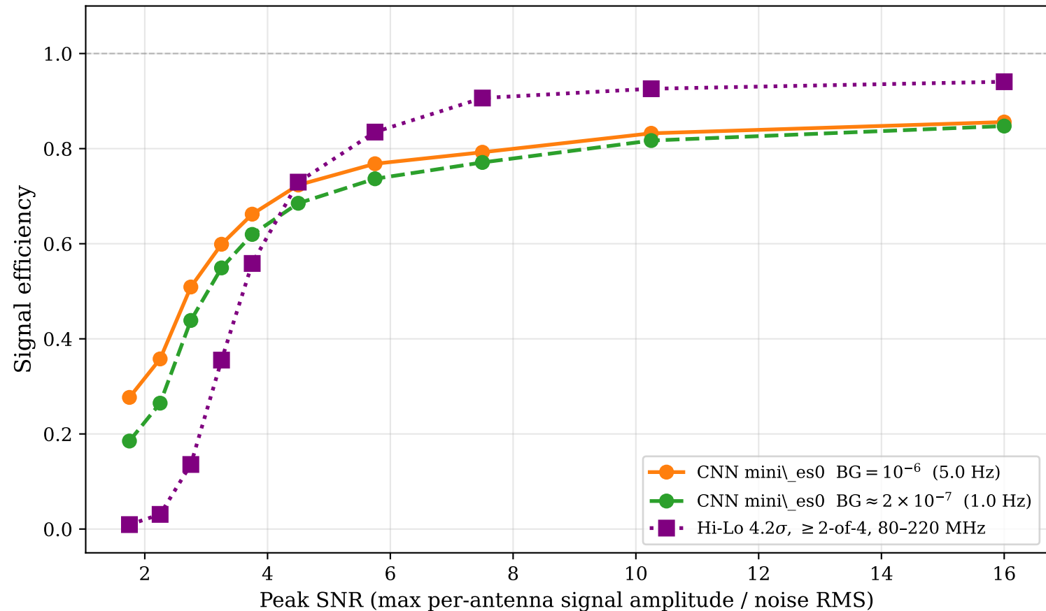
Efficiency vs. SNR — mini\_es0 CNN vs. Hi-Lo 4.2\sigma reference
