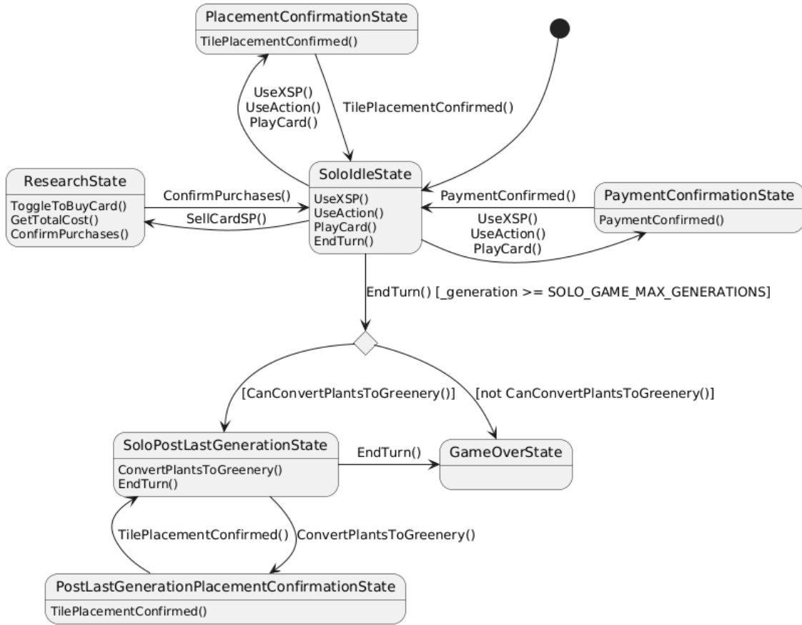
Figure 27: State diagram of the solo variant of the game.
