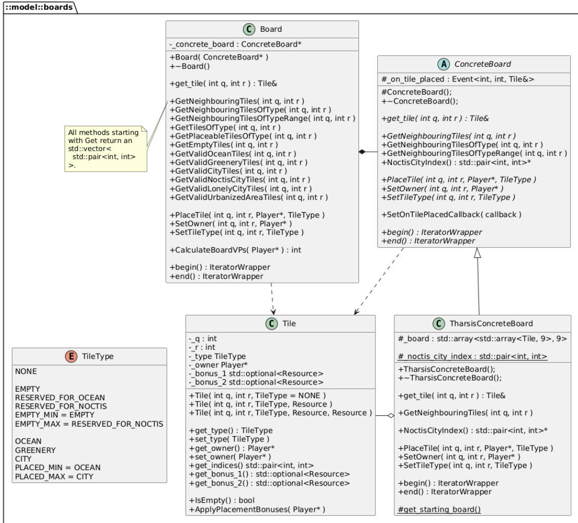
Figure 18: Class diagram of the ::model::boards namespace.
