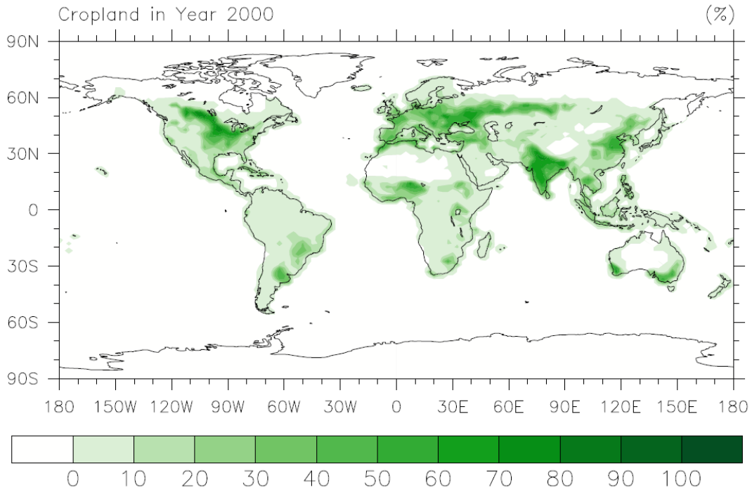
Figure S1: Cropland mask used to produce Figure 1 in the main text. Values are percent of each grid box used for crops. This is from land surface data of 2000 used in the Community Earth System Model. The resolution of this land file is 1 degree, and therefore along coastal lines and islands, the green color covers small parts of the ocean.
