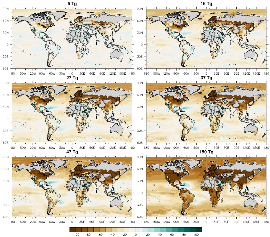
Figure S4. Change in calorie production (%) for the explicitly simulated agricultural crops and wild-caught marine fisheries combined. Percent change is for the nuclear war scenarios as compared to the control simulation, averaged for the first five years after the nuclear wars from the four cereals and marine fish we modeled. The dark green regions over the border area between India and Pakistan, and tropical dry regions, have close to zero crop yield in the control simulation with year 2000 climate forcing, and in CLM5crop, those areas have crop land percentage larger than 0 since the resolution is 1 degree. Therefore, those regions have small crop production in the control simulation. When the nuclear war perturbation is applied, those regions still show a low crop yield but higher than the control. Therefore, the percentage is positive and large.
