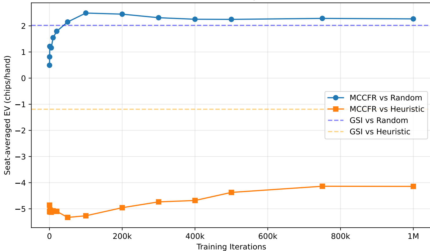
MCCFR Convergence
