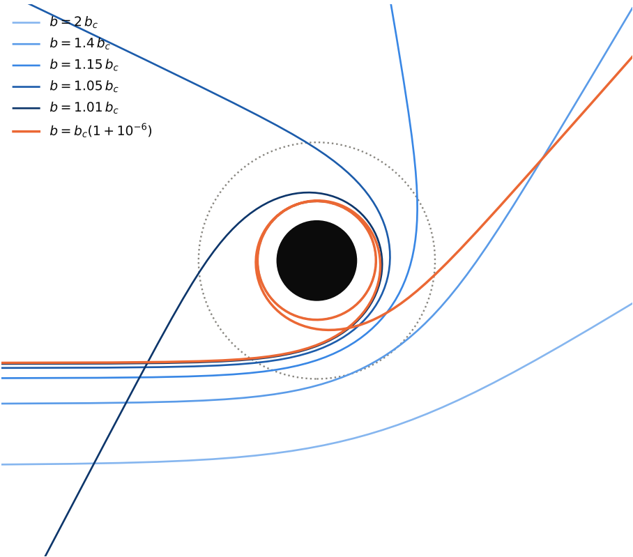
Light rays near the photon sphere
