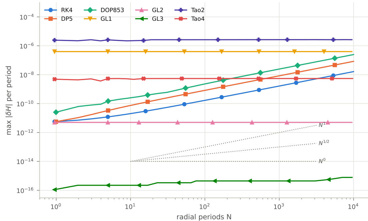
Mass-shell error over 10^4 periods of (20, 0.5), formulation (b)
