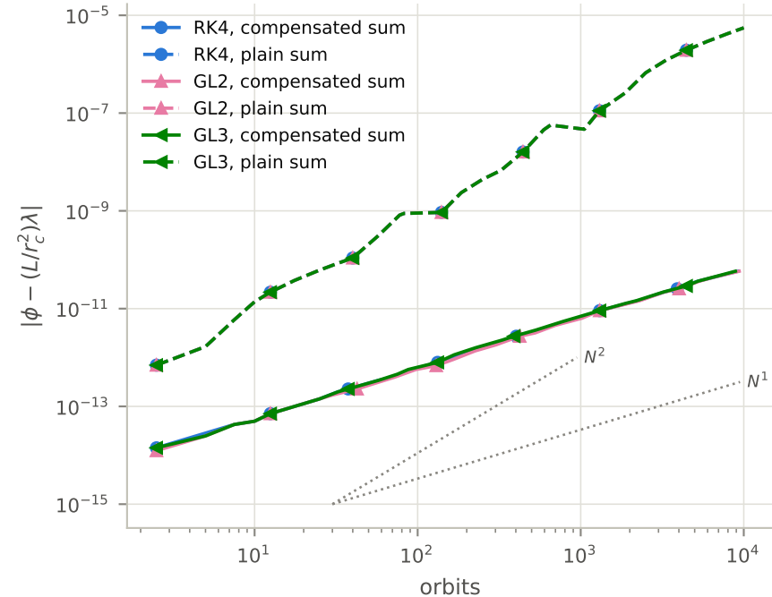
(i) circular r_c = 10 : phase from round-off alone (RK4, GL2, GL3 coincide)
