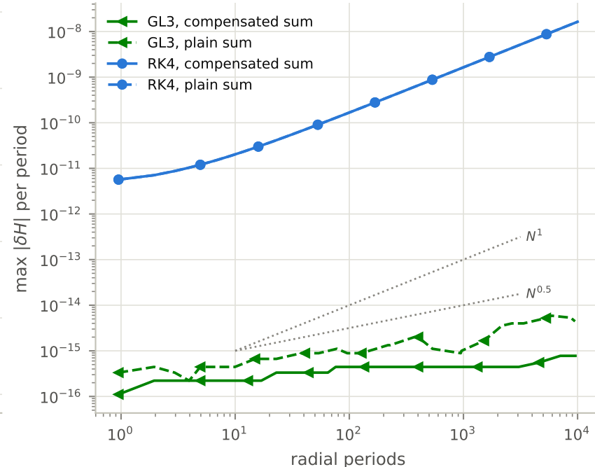
(ii) orbit (20, 0.5): mass shell
