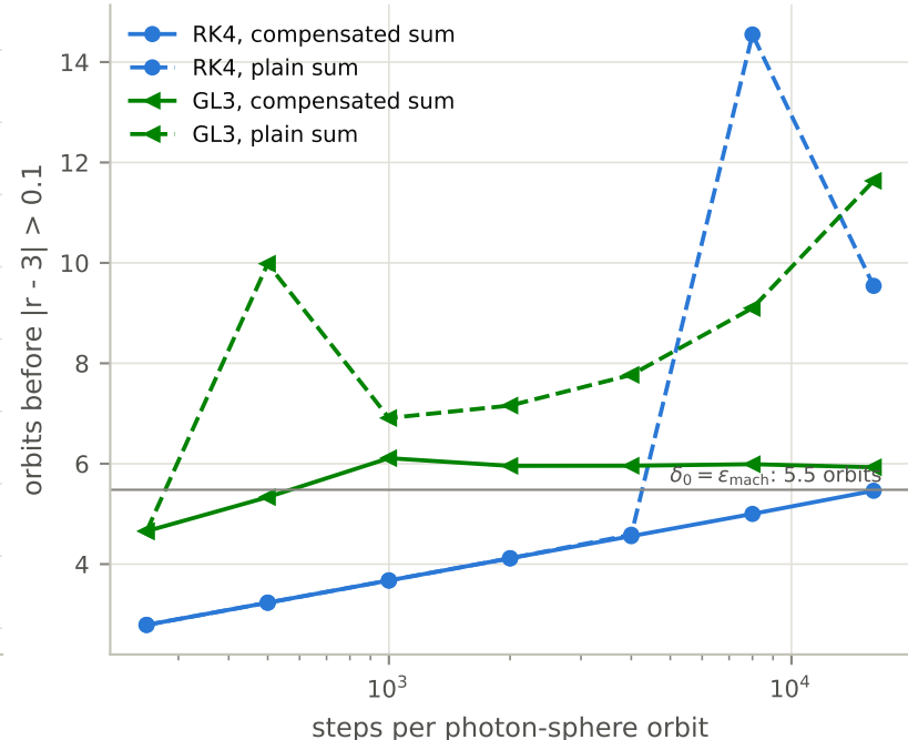
(iii) photon sphere, inclined 45^\circ (F10)
