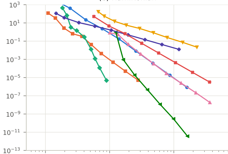
(b) Hamiltonian
