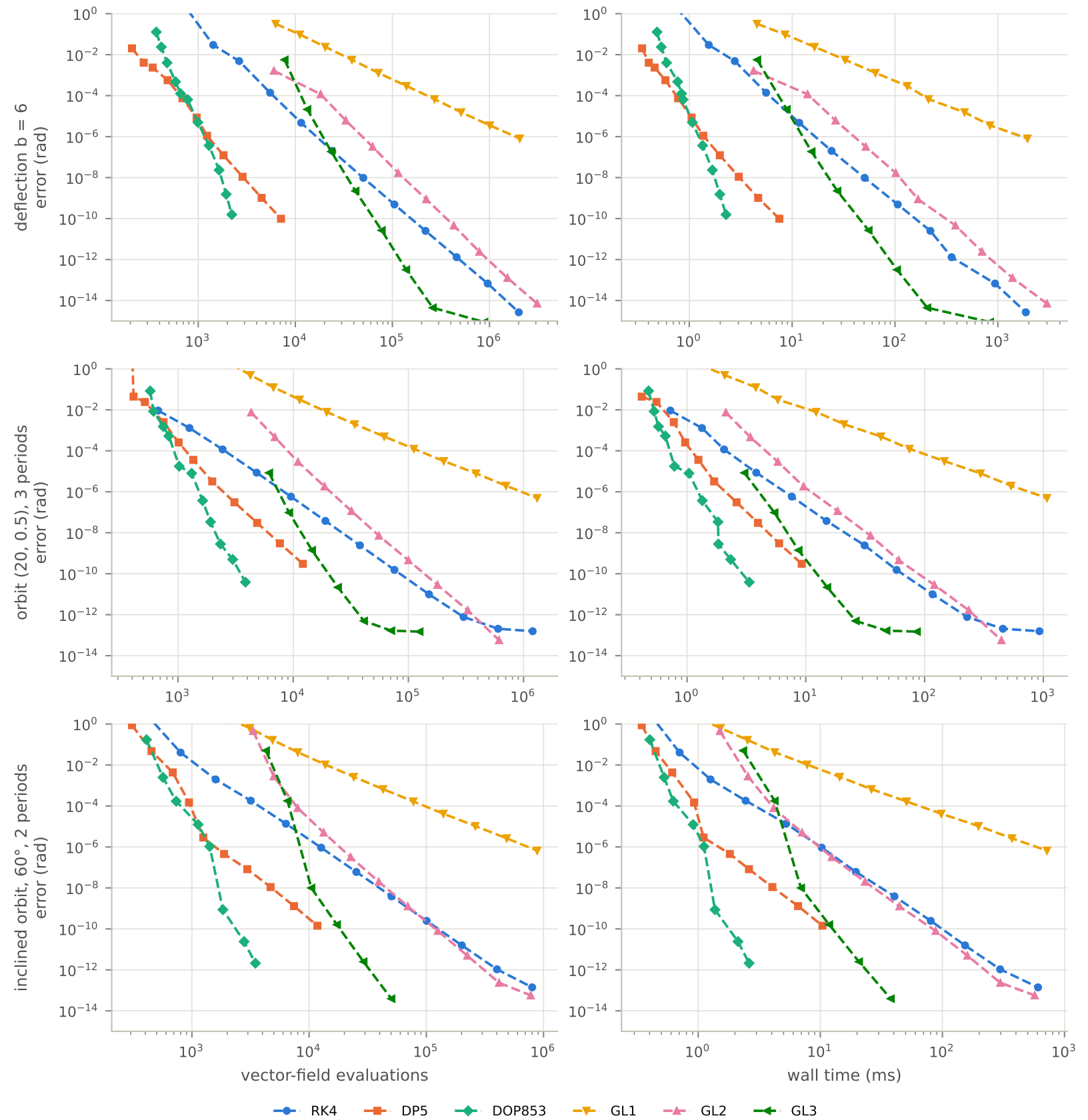
Work-precision, formulation (a) second order
