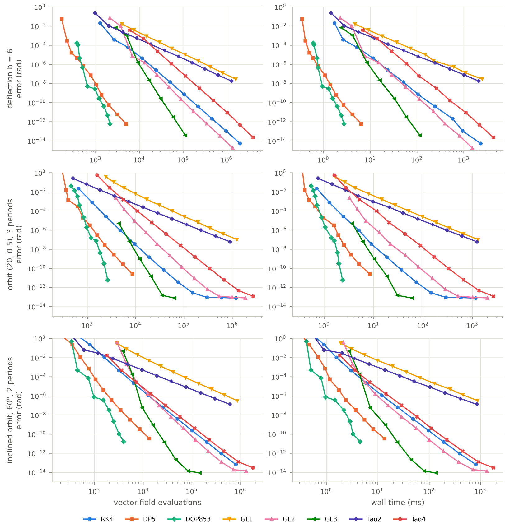
Work-precision, formulation (b) Hamiltonian
