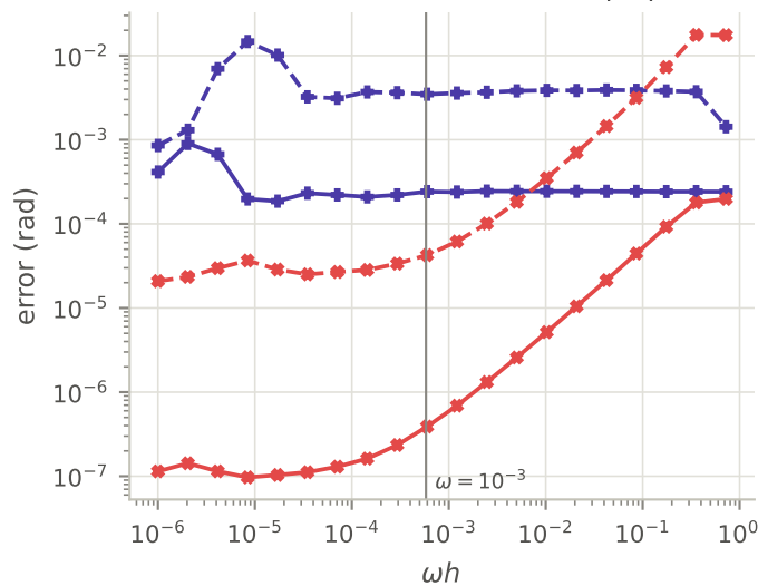
orbit (20, 0.5), 3 periods 400 (coarse) and 1600 (fine) steps/period
