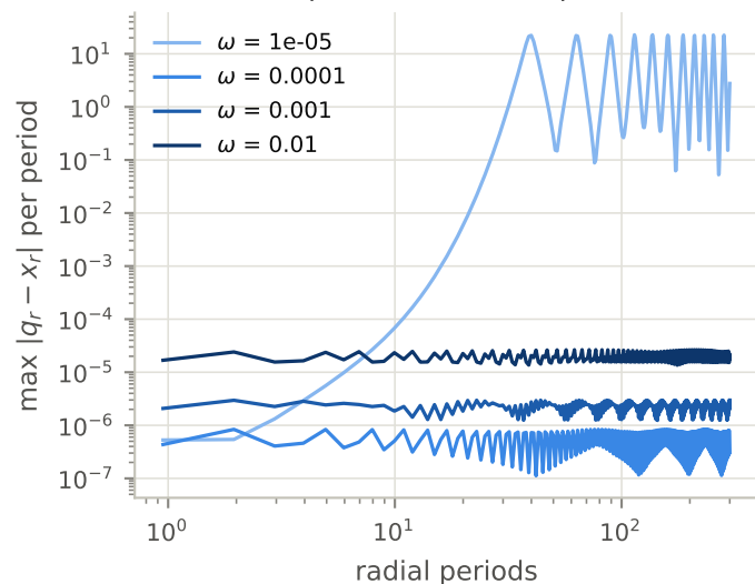
Tao4, 800 steps/period: separation of the copies
