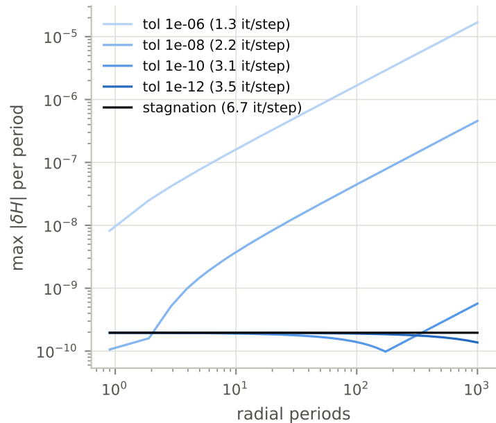
(iii) GL2, orbit (20, 0.5), 400 steps/period
