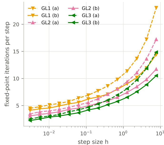
(i) orbit (7.5, 0.5)
