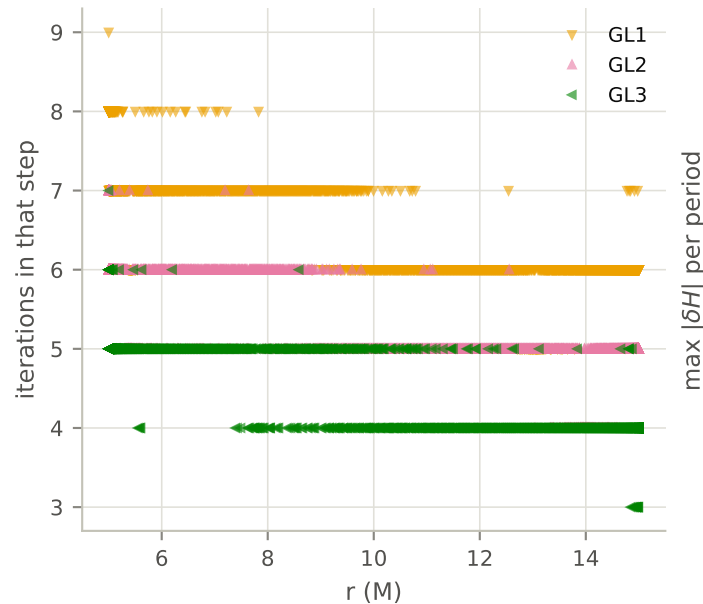
(ii) along the orbit, 2000 steps/period
