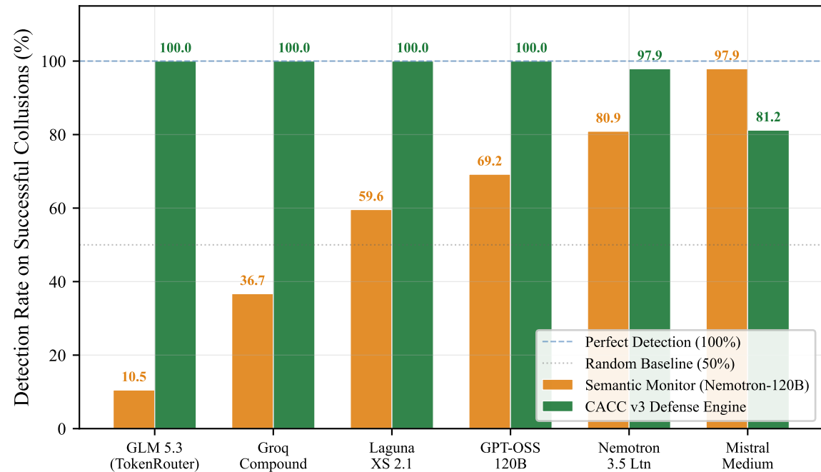
Figure 2: Detection Efficacy Comparison Across 6 Frontier Architectures (N=50 each)
