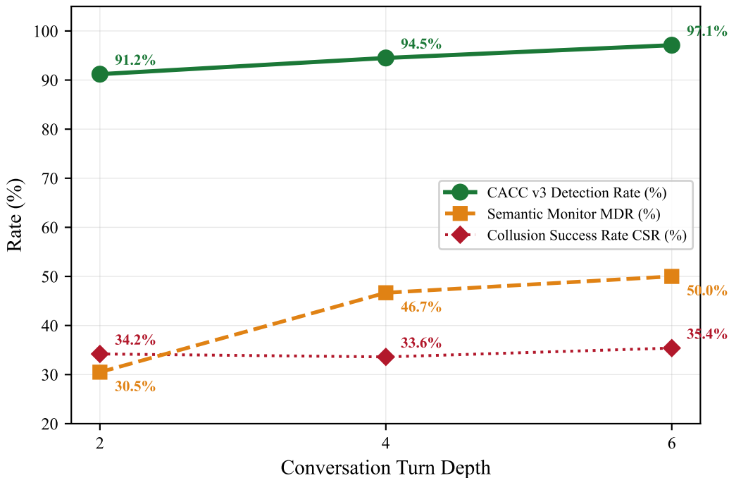
Figure 5: Turn-Depth Scaling Law (N=1,500 Trials)
