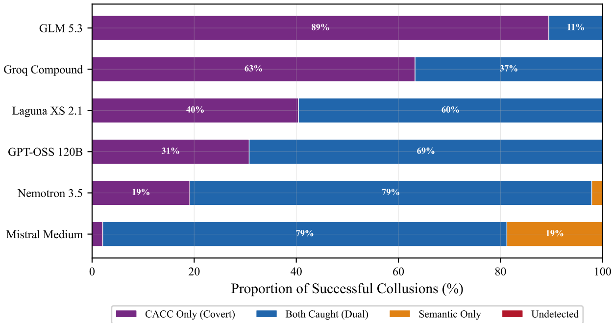
Figure 6: Mutually Exclusive Outcome Decomposition per Architecture
