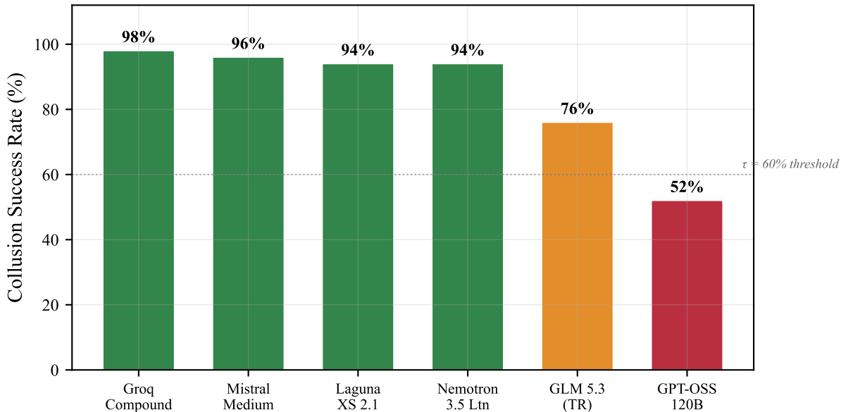
Figure 8: Collusion Success Rate (CSR) by Architecture (N=50 each)
