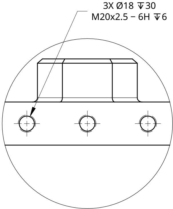
DETAIL A SCALE 2:5
