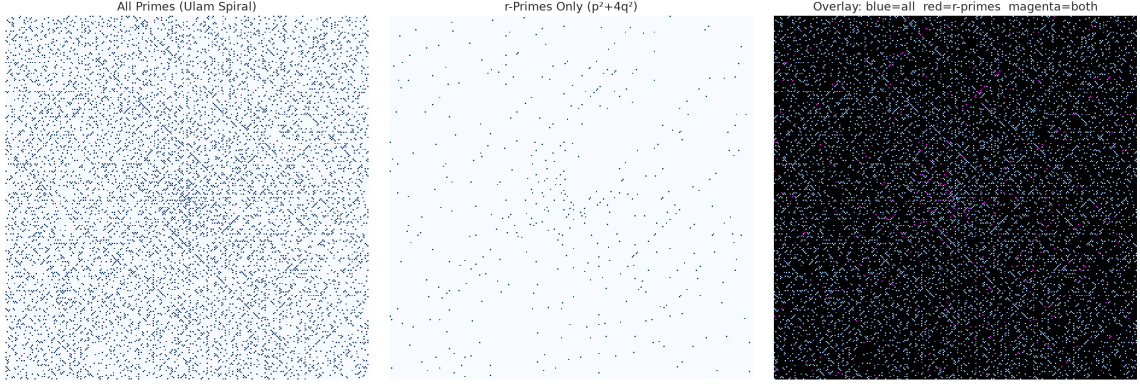
Figure 6: Ulam spiral (301×301). Left: all primes (blue). Center: R -primes only (red). Right: overlay, with magenta indicating overlap. The R -primes concentrate along diagonal bands.
