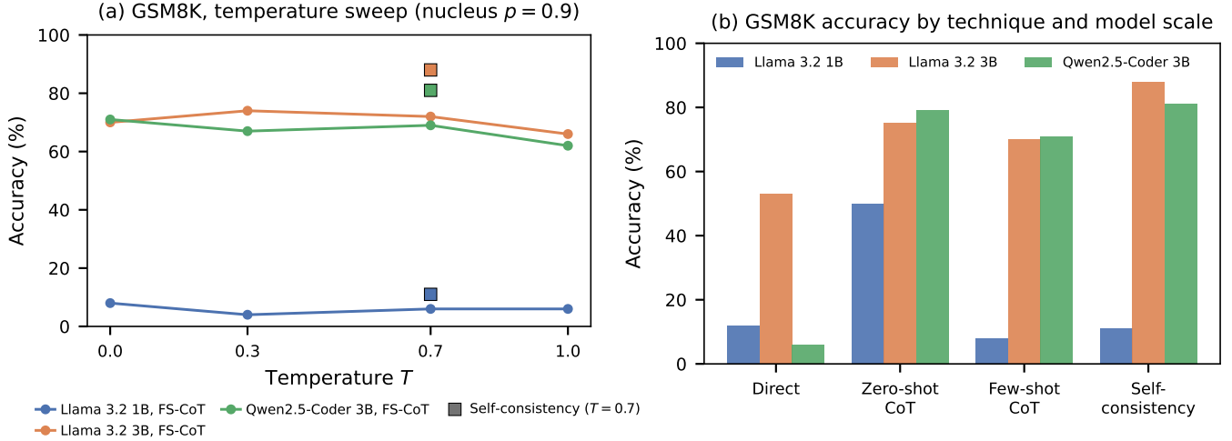
Fig. 1. (a) GSM8K accuracy versus temperature for single-sample few-shot CoT and self-consistency decoding under nucleus sampling ( p = 0.9 ); square markers at T = 0.7 denote self-consistency, which requires T > 0 and is evaluated at its defined setting T = 0.7 , while single-sample accuracy declines with temperature at the 1B and coder scales and is roughly flat at the 3B scale. (b) GSM8K accuracy by technique and model scale at the reference decoding cell; the zero-shot-CoT gain at the 1B scale (12% to 50%) is of the same order as the gain from scaling the model from 1B to 3B under direct answering (12% to 53%).
