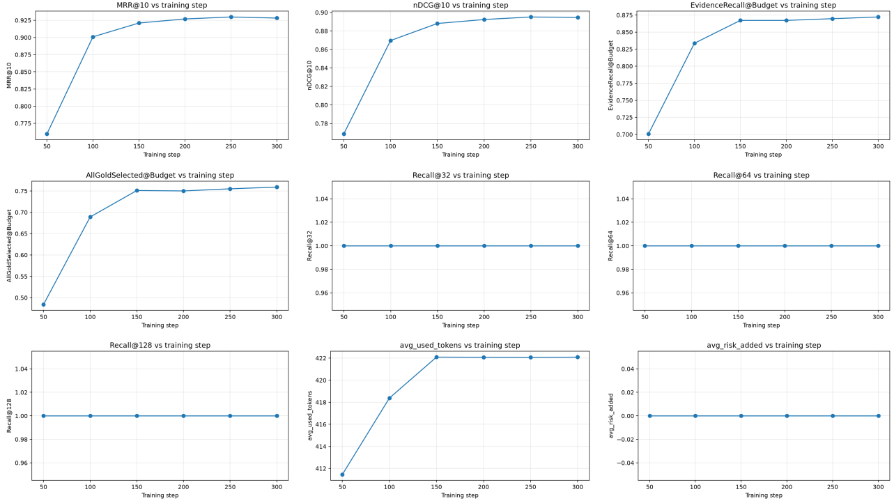
Figure 2: Metric curves across the six saved checkpoints.
