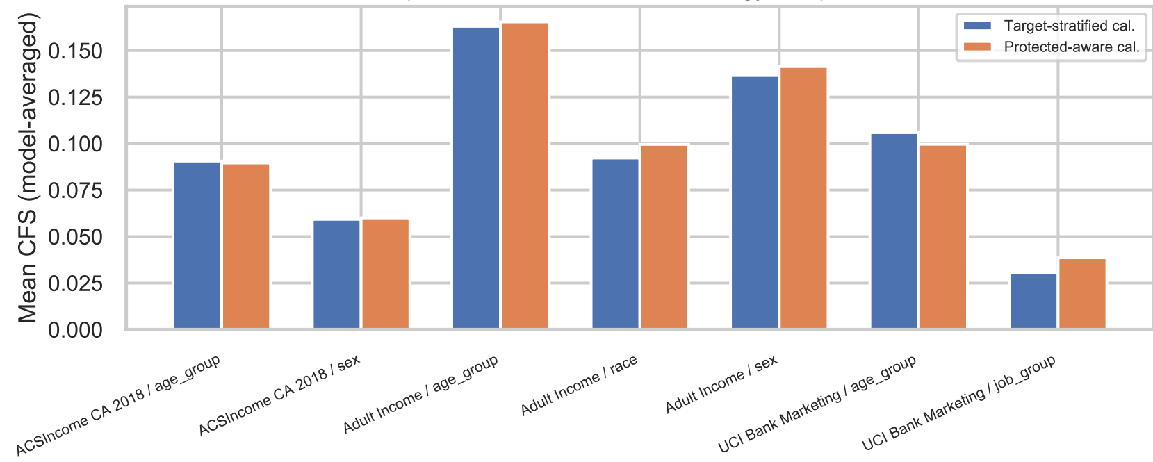
Equalized Odds: calibration strategy comparison
