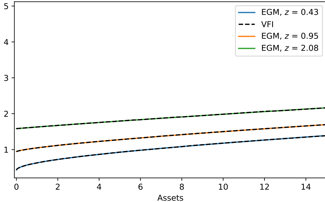
Consumption Policy Function
