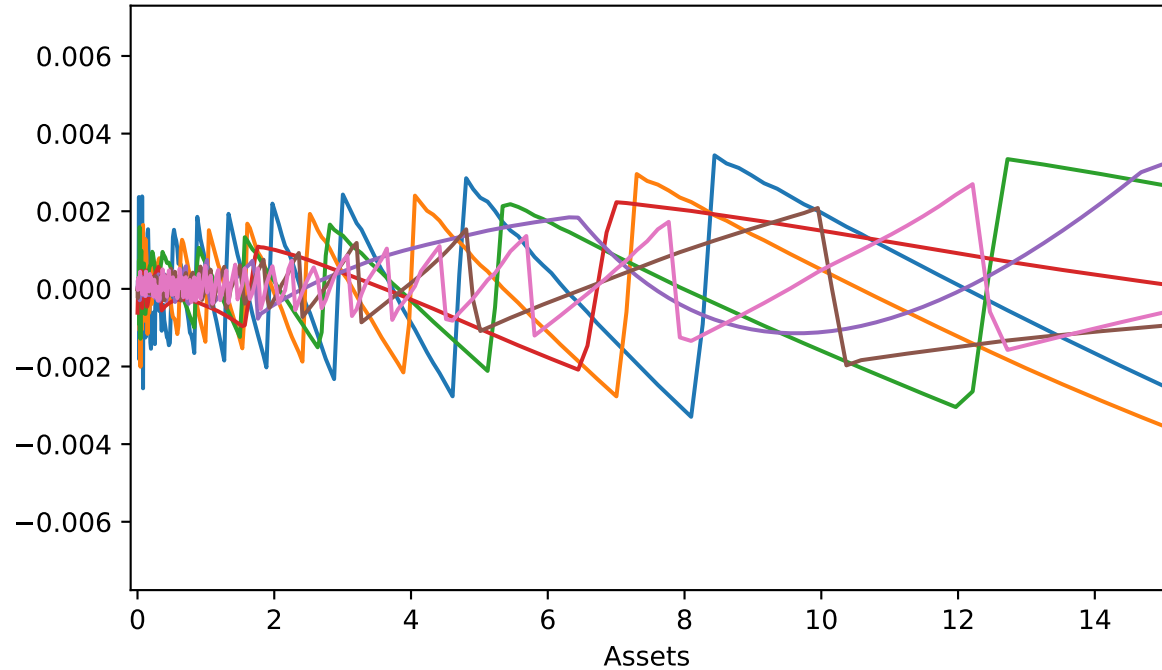
Relative difference, VFI vs EGM
