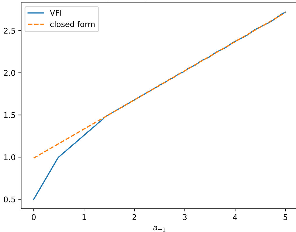
Consumption in period 0, rising income
