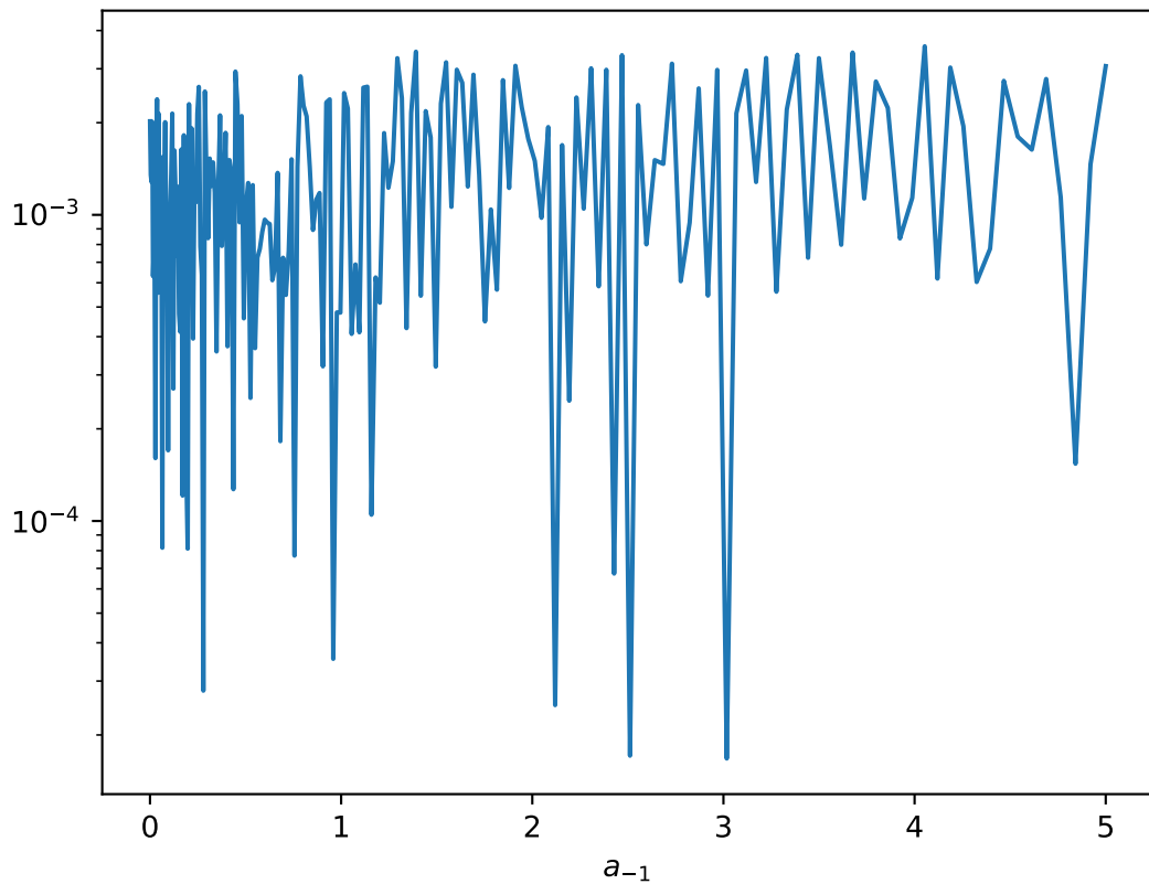
Relative error, VFI vs closed form
