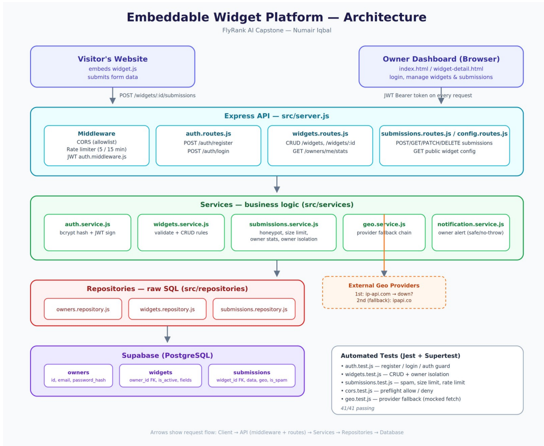
Figure 1: System architecture — embed script, public API, admin API, and PostgreSQL data layer.
